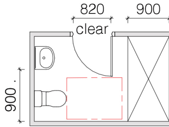
Figure 7 (e) Bathroom Design Option 5
